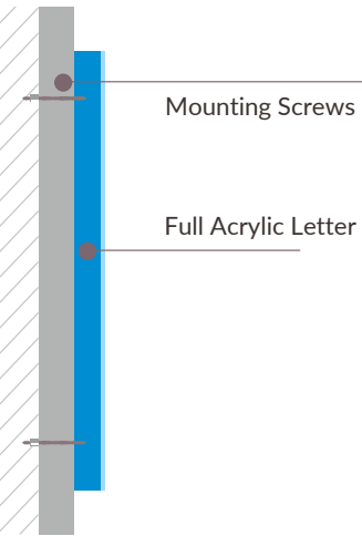
#2 Back-face Screws
